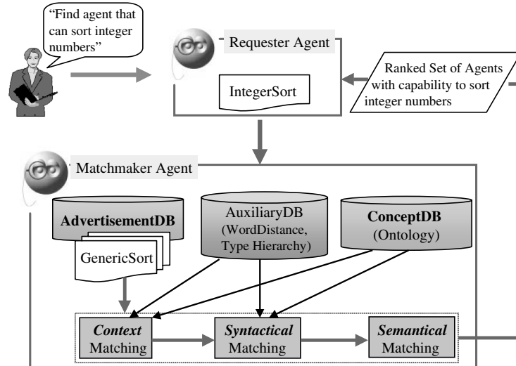
Figure 3. An example of matchmaking using LARKS.
